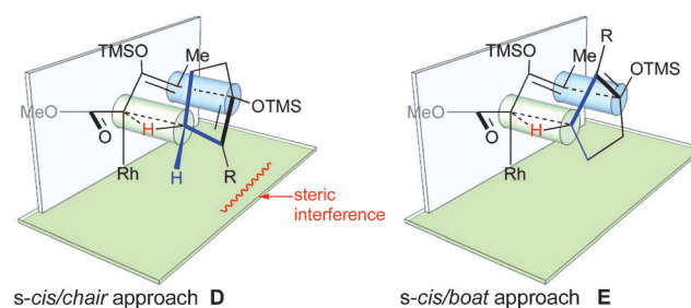
Figure 3. Transition state models for reaction of 1 with cyclopentenyls.
