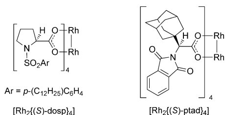
Scheme 2. Structures of [Rh_2\{(S)\text{-dosp}\}_4] and [Rh_2\{(S)\text{-ptad}\}_4] .
