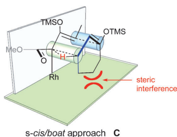
Figure 2. The s-cis/boat transition state model for the reaction of 1 with 2 .
