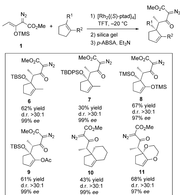
Scheme 3. The CHCR reactions with cyclopentenyl derivatives. TBS = tert -butyldimethylsilyl, TBDPS = tert -butyldiphenylsilyl.
